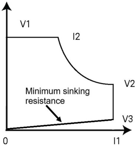
Figure 9. EL4900 characteristic
